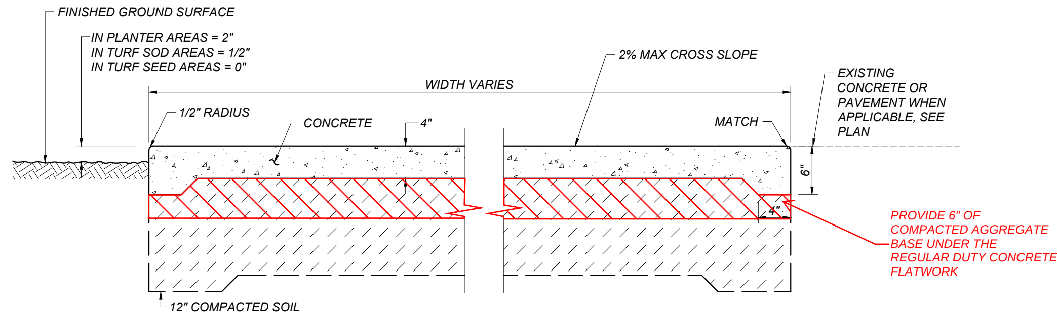
A REGULAR-DUTY CONCRETE X100 NOT TO SCALE
