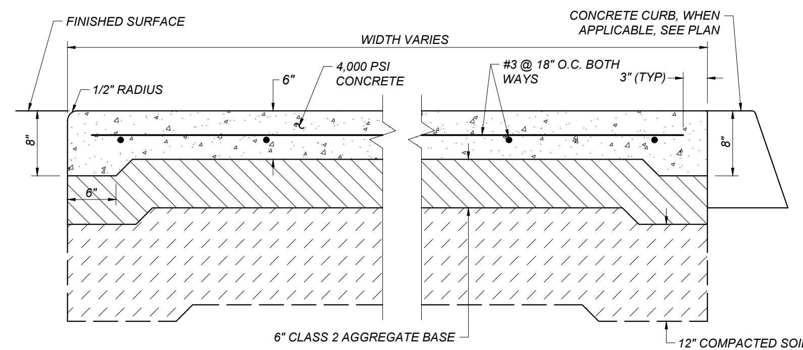
J HEAVY DUTY CONCRETE PAVEMENT STRUCTURAL SECTION X100 NOT TO SCALE
