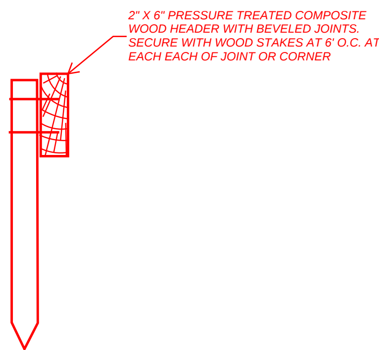
L PRESSURE TREATED HEADER X100
