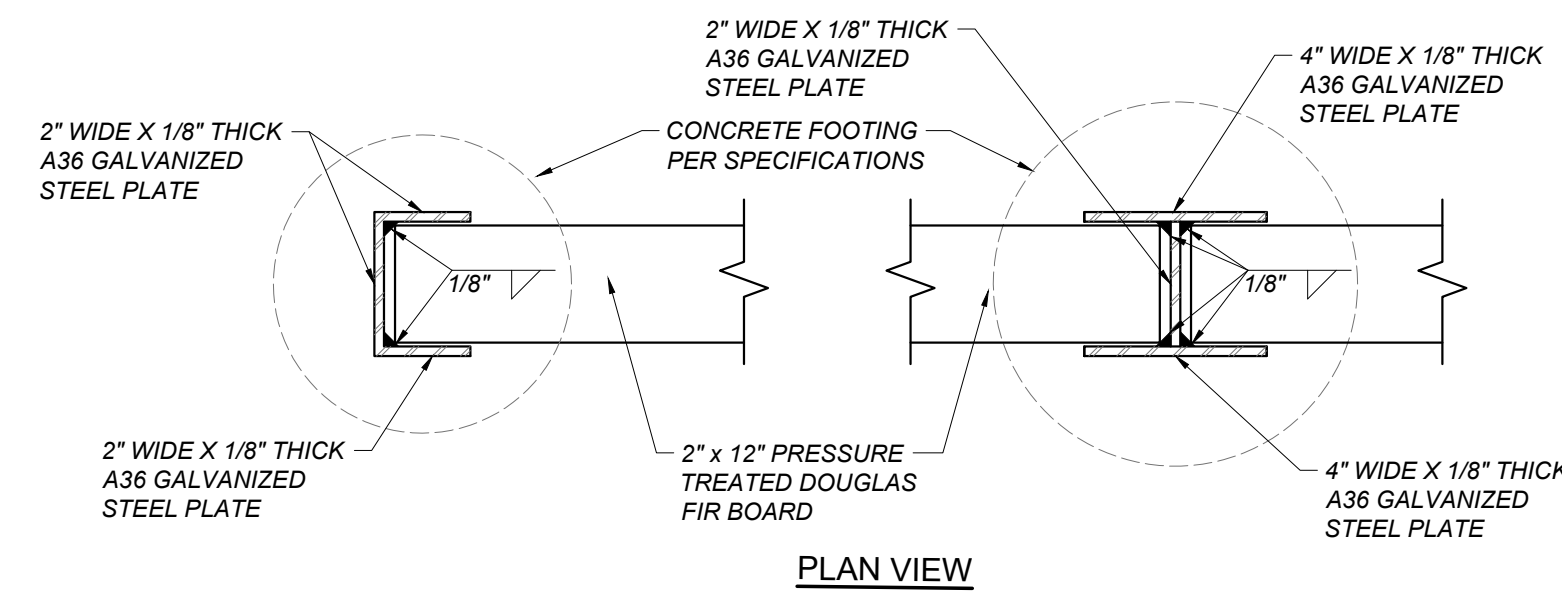
K MATERIAL STORAGE BAY WOOD WALL X100 NOT TO SCALE NOTE: THIS WORK IS EXEMPT FROM DSA STRUCTURAL SAFETY AND FIRE LIFE SAFETY REVIEW PER DSA IR A-22 SECTION 1.2.1
